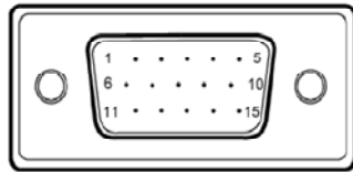
15-Pin Color Display Signal Cable
