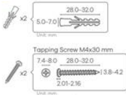
Figure 3 Screw Specifications
