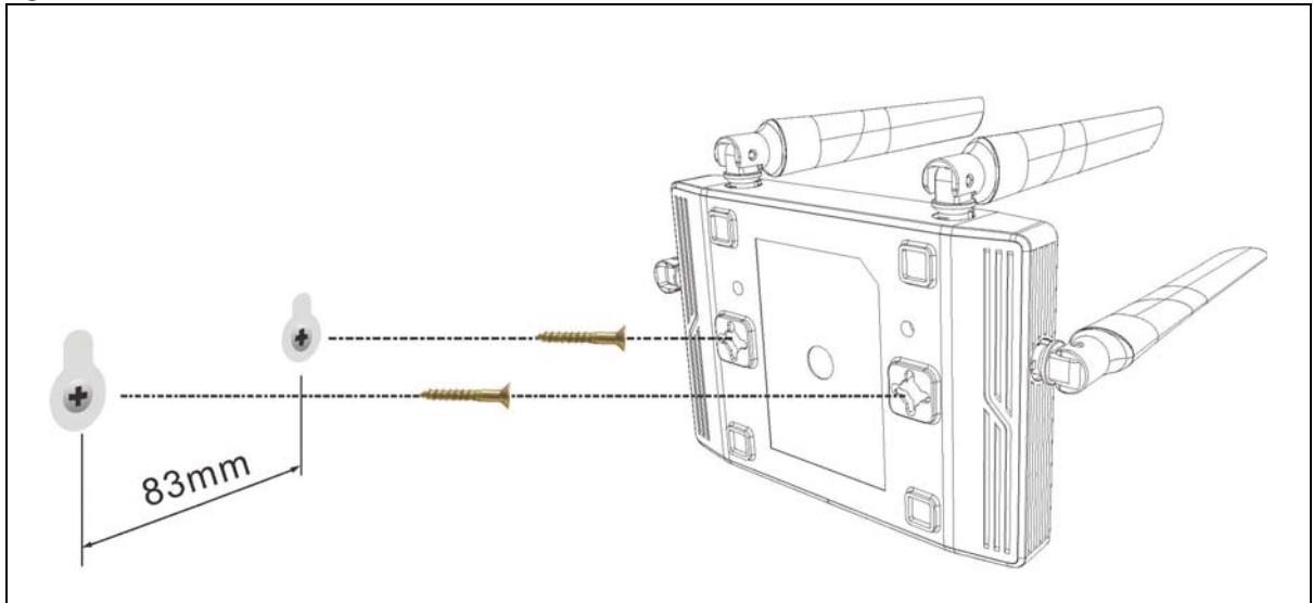
Figure 4 Wall Mounting Example
