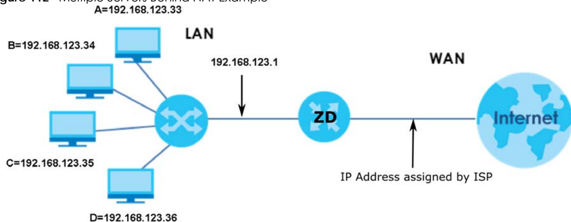
Figure 112 Multiple Servers Behind NAT Example
