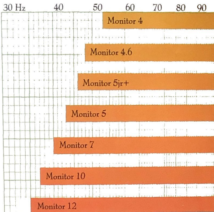
Low Frequency Limit at -3 dB for each Monitor shows increased bass performance as you move up in size.
