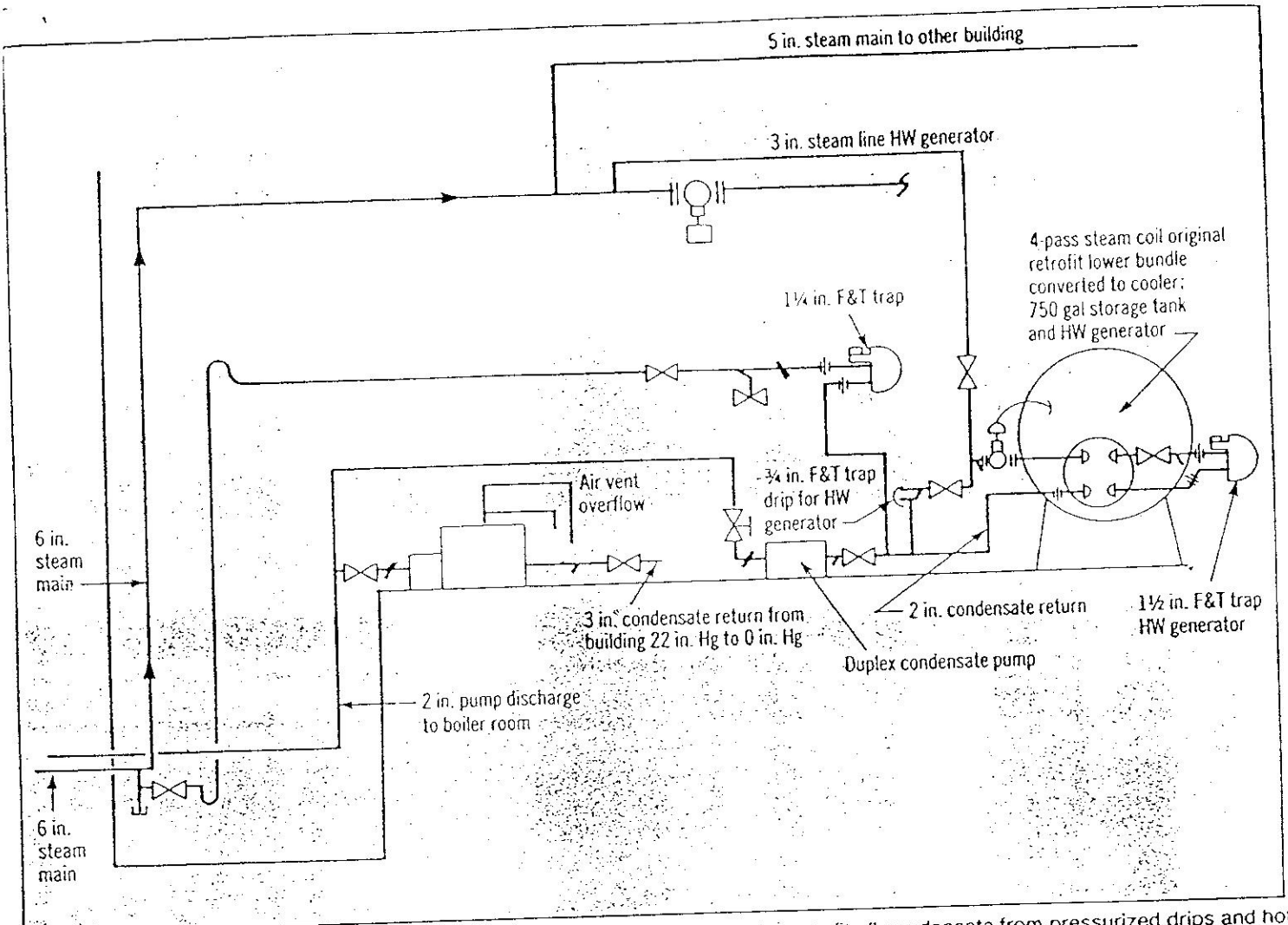
3 Corrected method of condensate removal employing the steam siphon. During retrofit all condensate from pressurized drips and hot water generator was relocated to new condensate pump. The heating system was totally separated from hot water generator and all drips, thereby eliminating any source of hot condensate from affecting the operation of variable vacuum operation.
