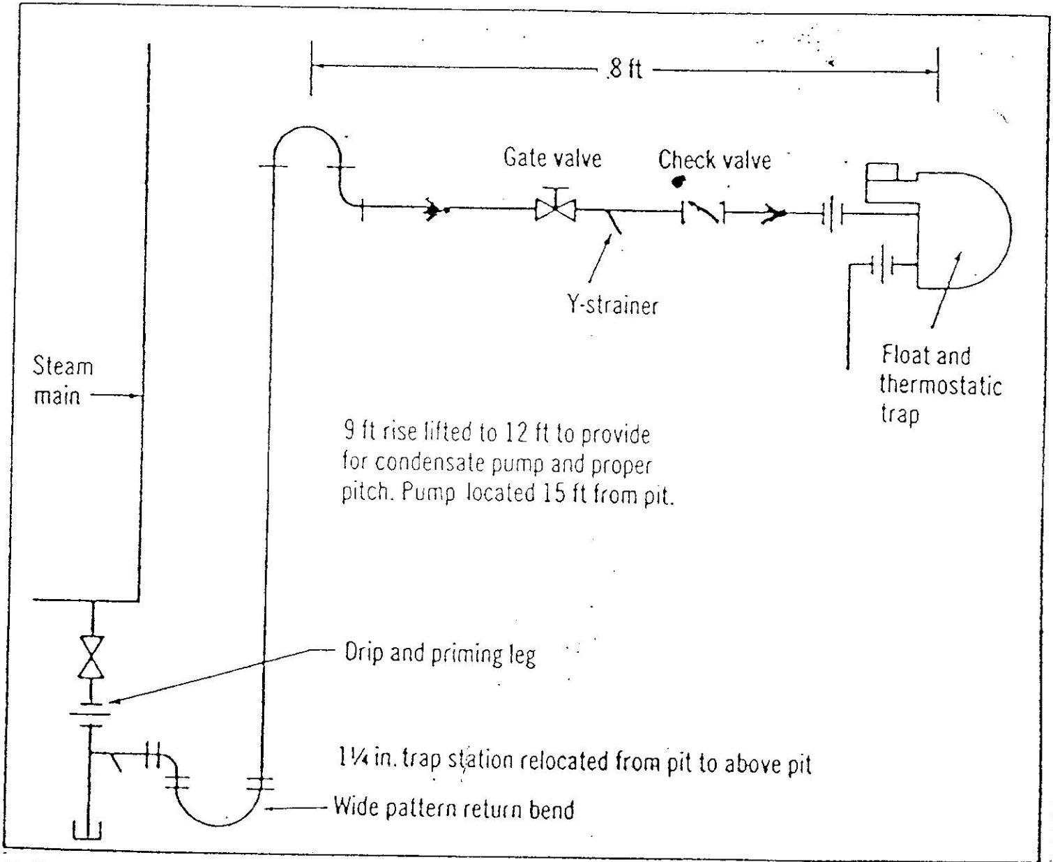
2 Steam siphon.
