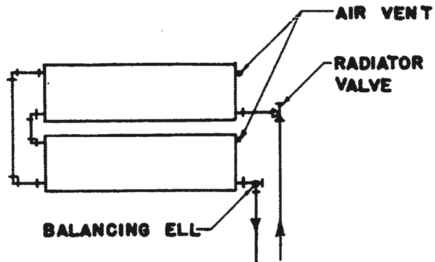
SUPPLY & RETURN AT SAME END OF ASSEMBLY
