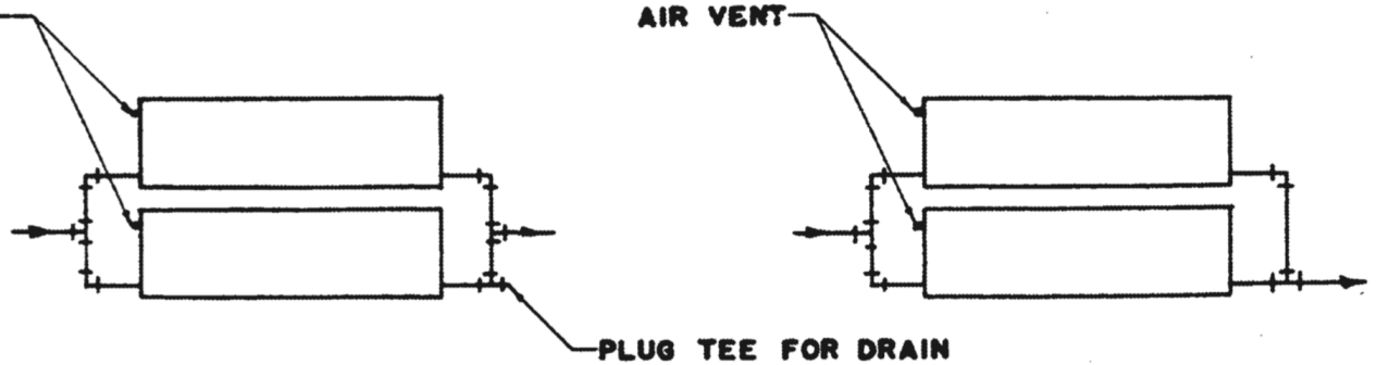
SUPPLY & RETURN AT OPPOSITE ENDS OF ASSEMBLY
