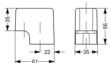
Compact-adapter for wall temperature adjusters
