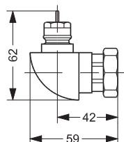
Angle adapter 013G1360 for M30x1,5 connection
