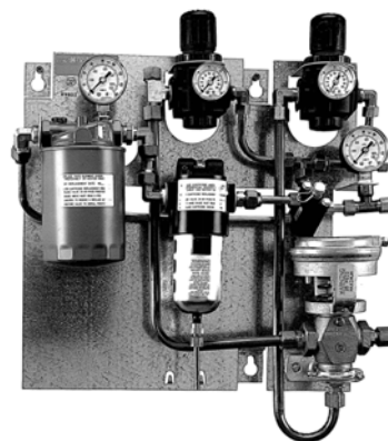
Fig. 2: A-4000-140 10 SCFM, Dual PRV Station
