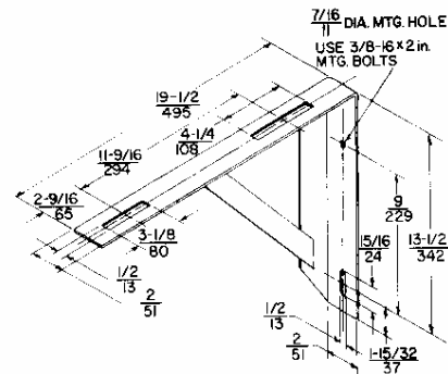
Fig. 19: A-4000-108 Wall Bracket (1/8 in. Plate Metal)
