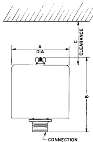
Fig. 25: Dimensions (in./mm) (See Table 6.)
