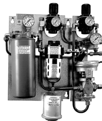
Fig. 4: A-4000-142 20 SCFM, Dual PRV Station (Shown with Optional Oil Reservoir)
