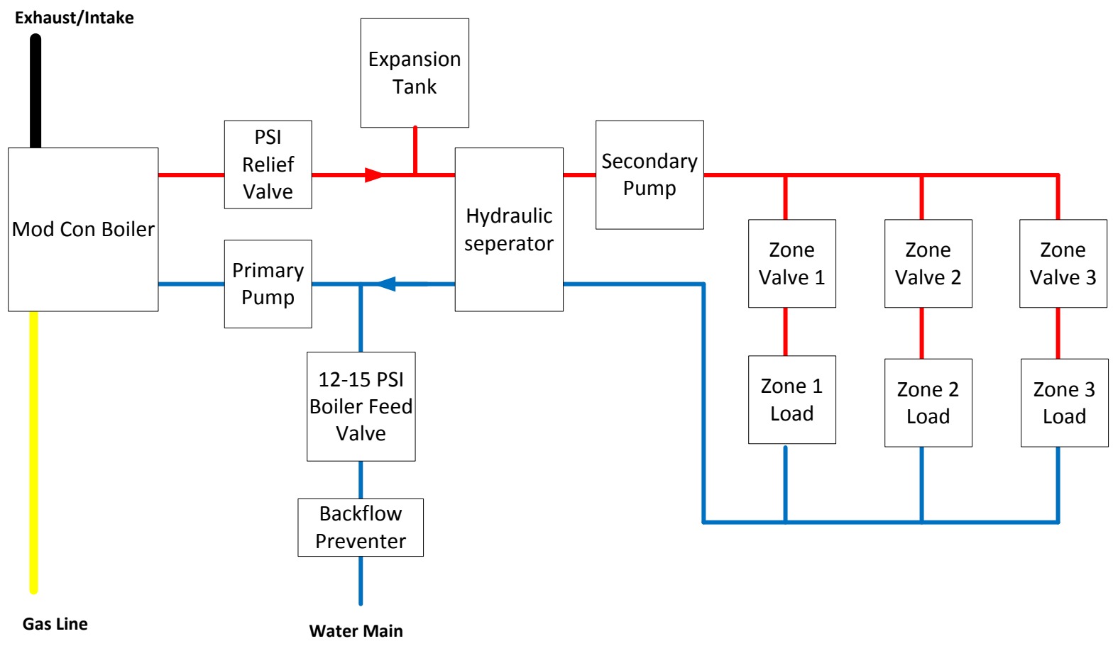
Primary/Secondary Piping
