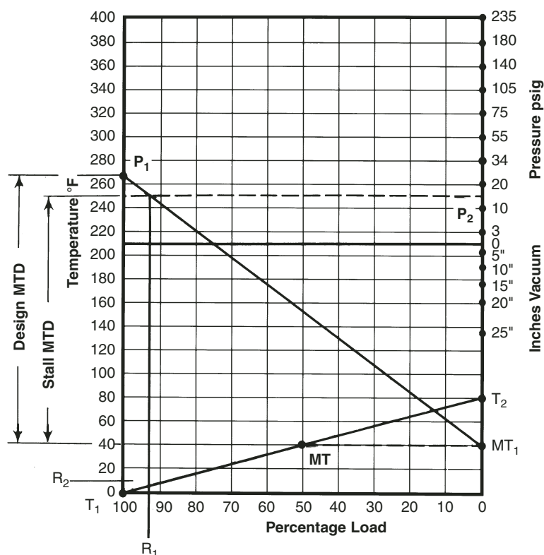
Figure 46: Air Make-up Coil Stall Chart
