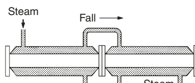
Figure 12b Jacketed Lines, Connected
