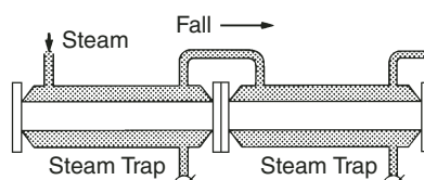
Figure 12a Jacketed Lines, Drained Separately
