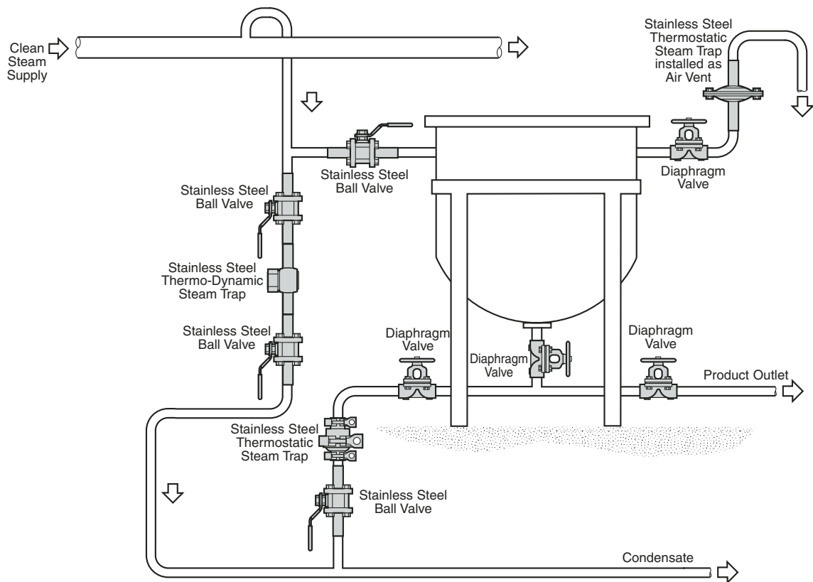
Figure II-87 Tank Sterilization
