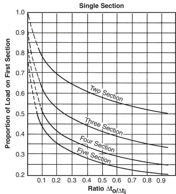
Figure 50 Load on First Section of Multi-Coil Heater
