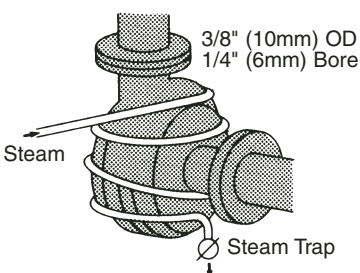
Figure 31 Tracer Lines Around Pump Casing
