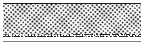
Figure 10b Continuous Weld
