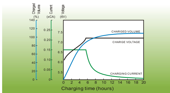
Constant voltage charging characteristic (0.15CA, 25°C, 77°F)
