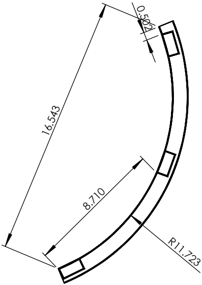
SECTION E-E SCALE 1 : 6
