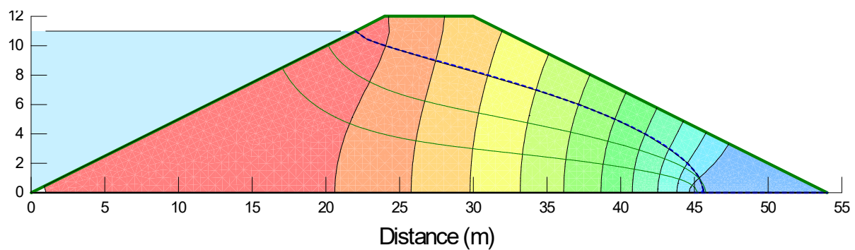
Figure 3. SEEP/W results.
